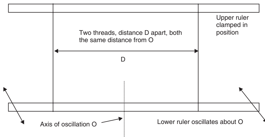
Fig.2-3; Bifilar suspension
